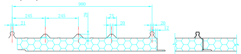
Nips matching roof plate: 980mm EPS core
