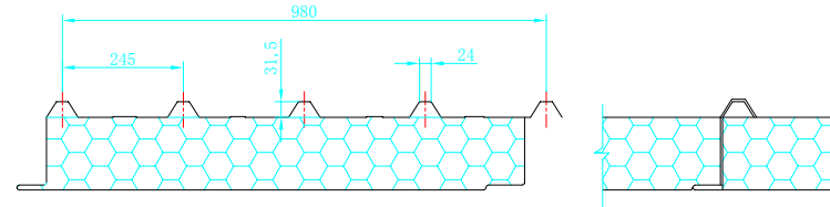
Cap roof plate:950mm EPS core
