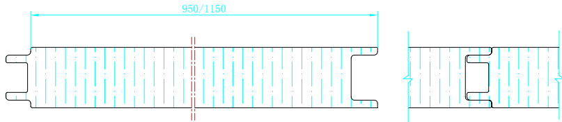
Double cap roof plate: 980mm EPS core
