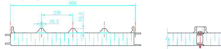
Nips matching roof plate: 950mm EPS core
