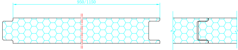
infixing panel:1150/950mm Rock wool core
