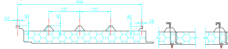
Nips matching roof plate: 950mm EPS core
