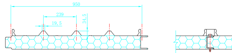
infixing roof plate:950mm Rock wool core
