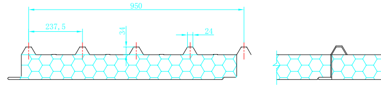
Joint roof plate: 980mm EPS core
