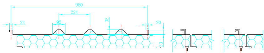
Nips matching roof plate: 980mm EPS core
