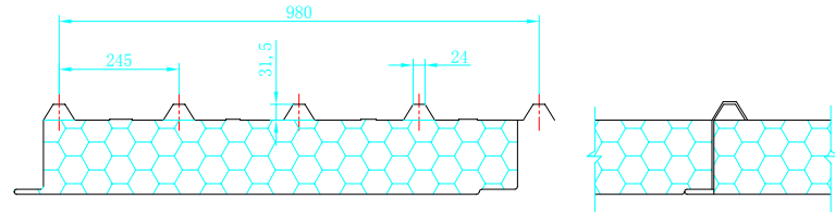
Cap roof plate:950mm EPS core
