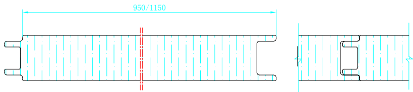
infixing panel:1150/950mm Rock wool core
