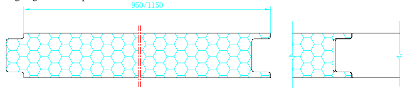
Hidden wall panel:1125mm EPS core
