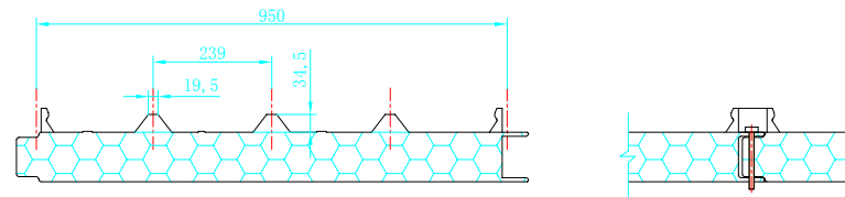
Cap roof plate:950mm Rock wool core
