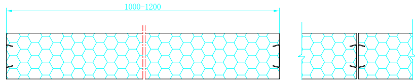
tong & groove wall panel: 1150/950mm EPS core
