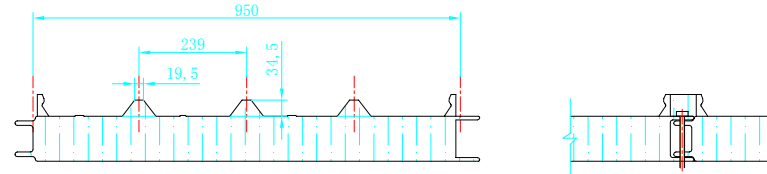
Cap roof plate:950mm Rock wool core
